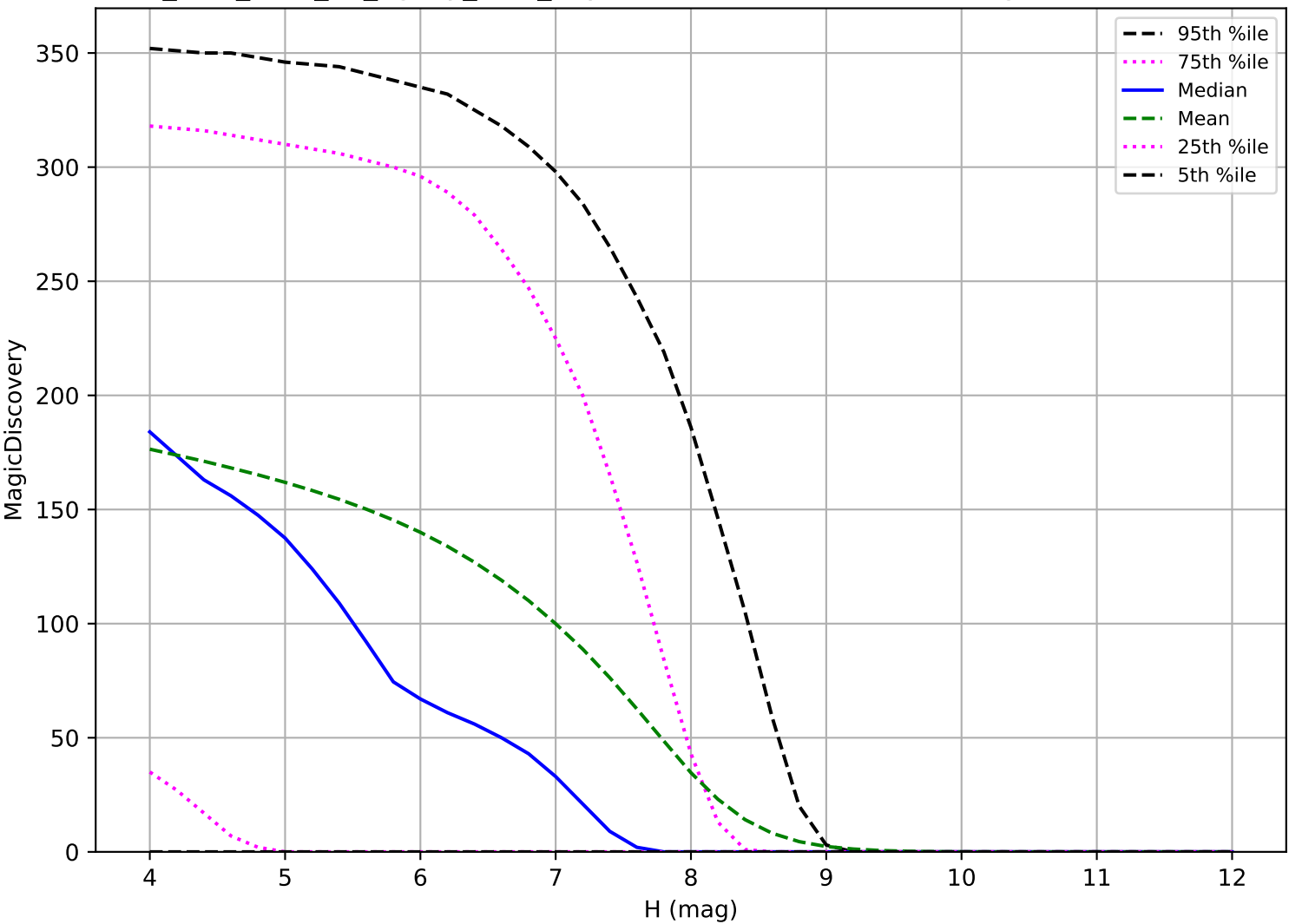
too_elab_r128_d2_ugrizy_v3.4_10yrs: TNO 6 detections in 60 nights detection loss
