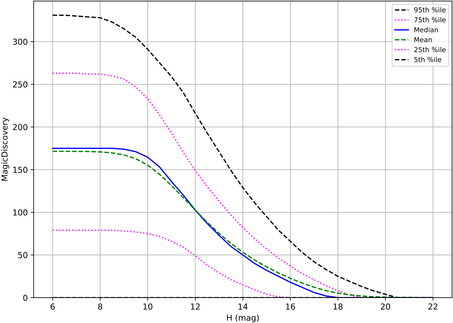
too_elab_r128_d2_ugrizy_v3.4_10yrs: OCC_r5 6 detections in 60 nights detection loss
