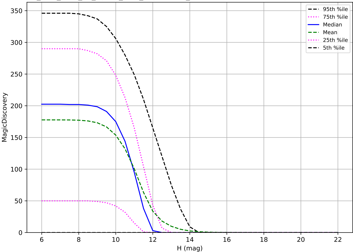
too_elab_r128_d2_ugrizy_v3.4_10yrs: OCC_r20 6 detections in 60 nights detection loss
