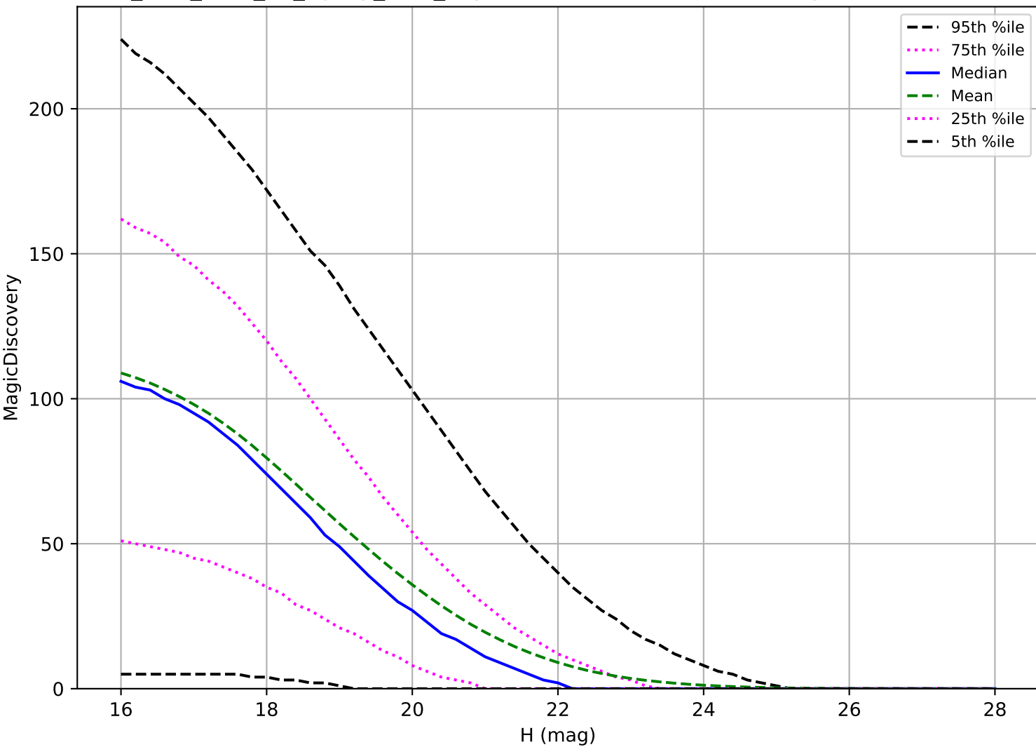
too_elab_r128_d2_ugrizy_v3.4_10yrs: NEO 6 detections in 60 nights detection loss
