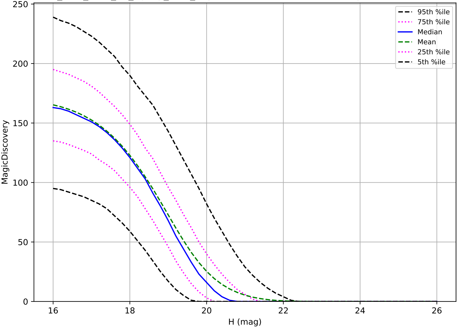
too_elab_r128_d2_ugrizy_v3.4_10yrs: MBA 6 detections in 60 nights detection loss
