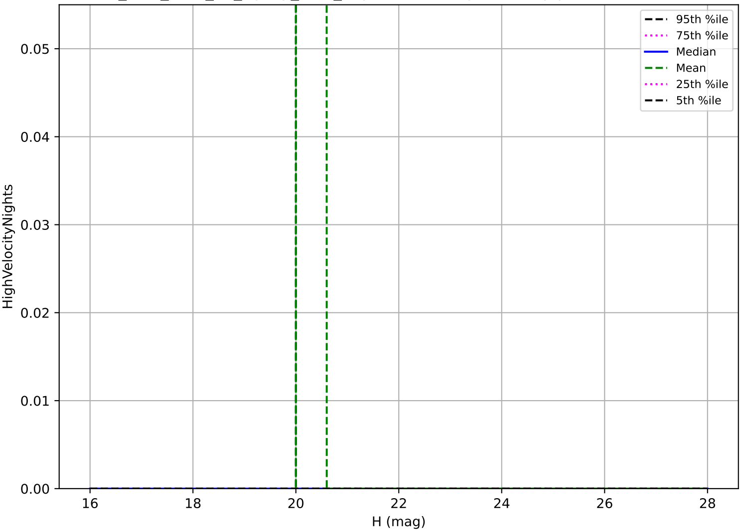
too_elab_r128_d2_ugrizy_v3.4_10yrs: Vatira High velocity pair detection loss
