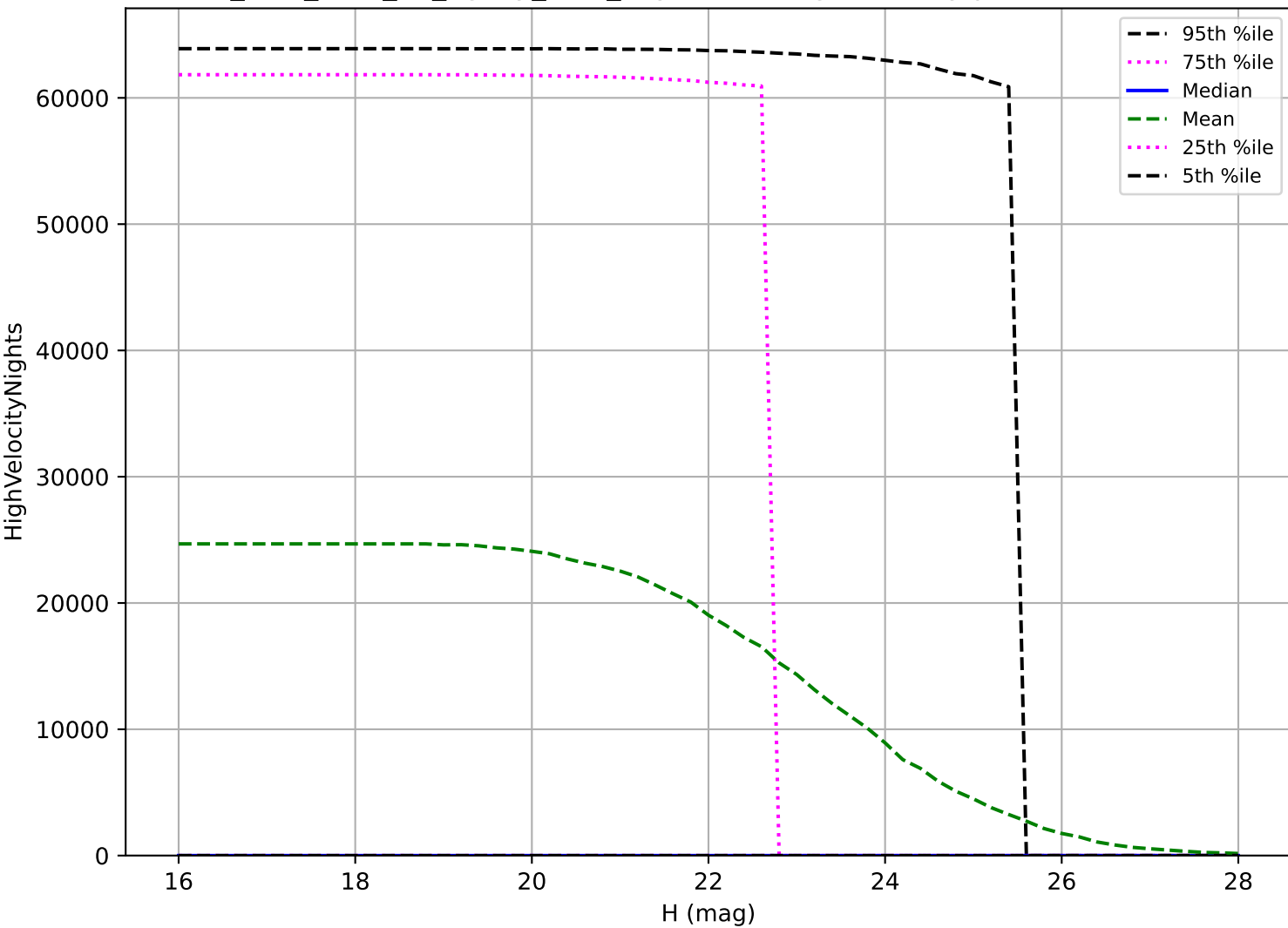
too_elab_r128_d2_ugrizy_v3.4_10yrs: PHA High velocity pair detection loss
