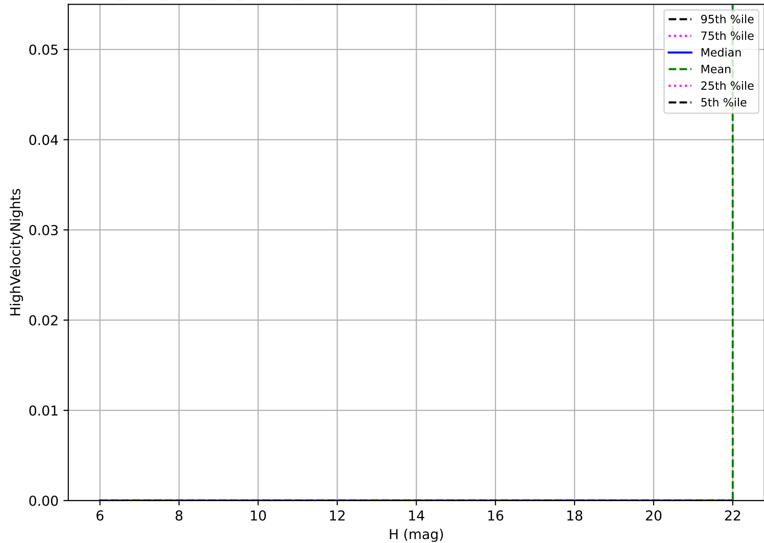
too_elab_r128_d2_ugrizy_v3.4_10yrs: OCC_r20 High velocity pair detection loss
