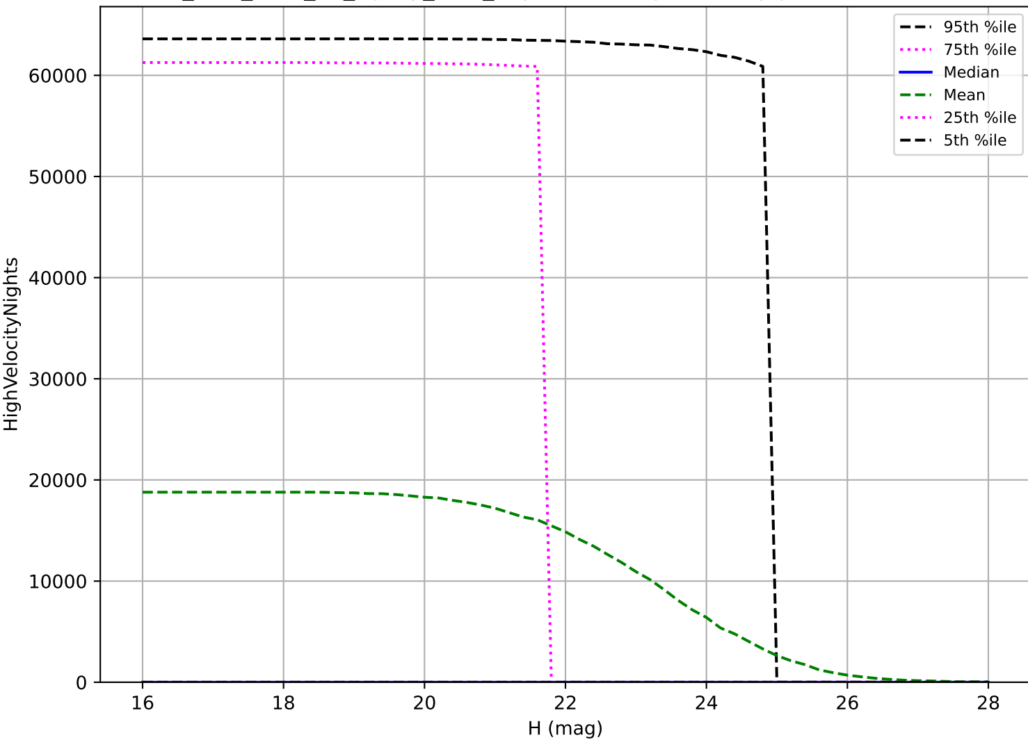
too_elab_r128_d2_ugrizy_v3.4_10yrs: NEO High velocity pair detection loss
