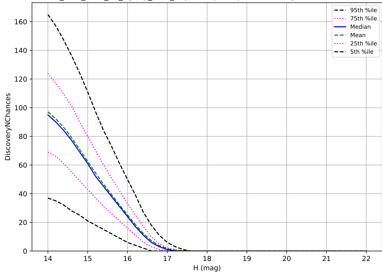
too_elab_r128_d2_ugrizy_v3.4_10yrs: Trojan 3 pairs in 15 nights detection loss
