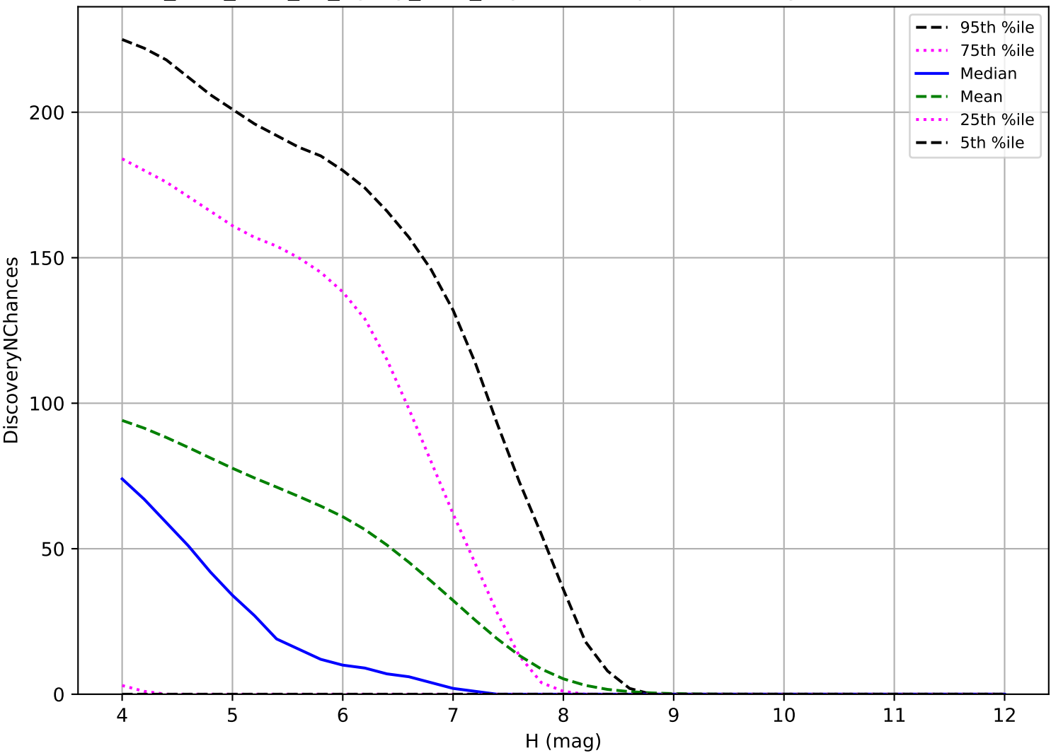
too_elab_r128_d2_ugrizy_v3.4_10yrs: TNO 3 pairs in 15 nights detection loss
