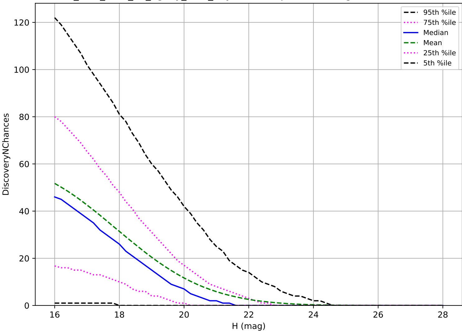
too_elab_r128_d2_ugrizy_v3.4_10yrs: PHA 3 pairs in 15 nights detection loss
