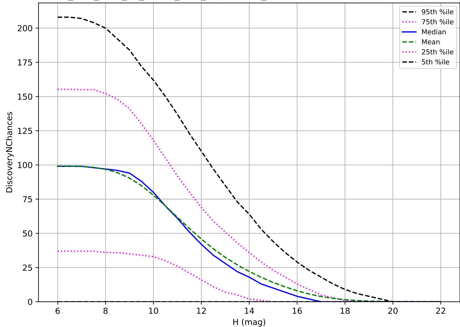
too_elab_r128_d2_ugrizy_v3.4_10yrs: OCC_r5 3 pairs in 15 nights detection loss
