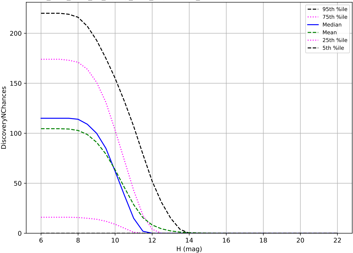
too_elab_r128_d2_ugrizy_v3.4_10yrs: OCC_r20 3 pairs in 15 nights detection loss
