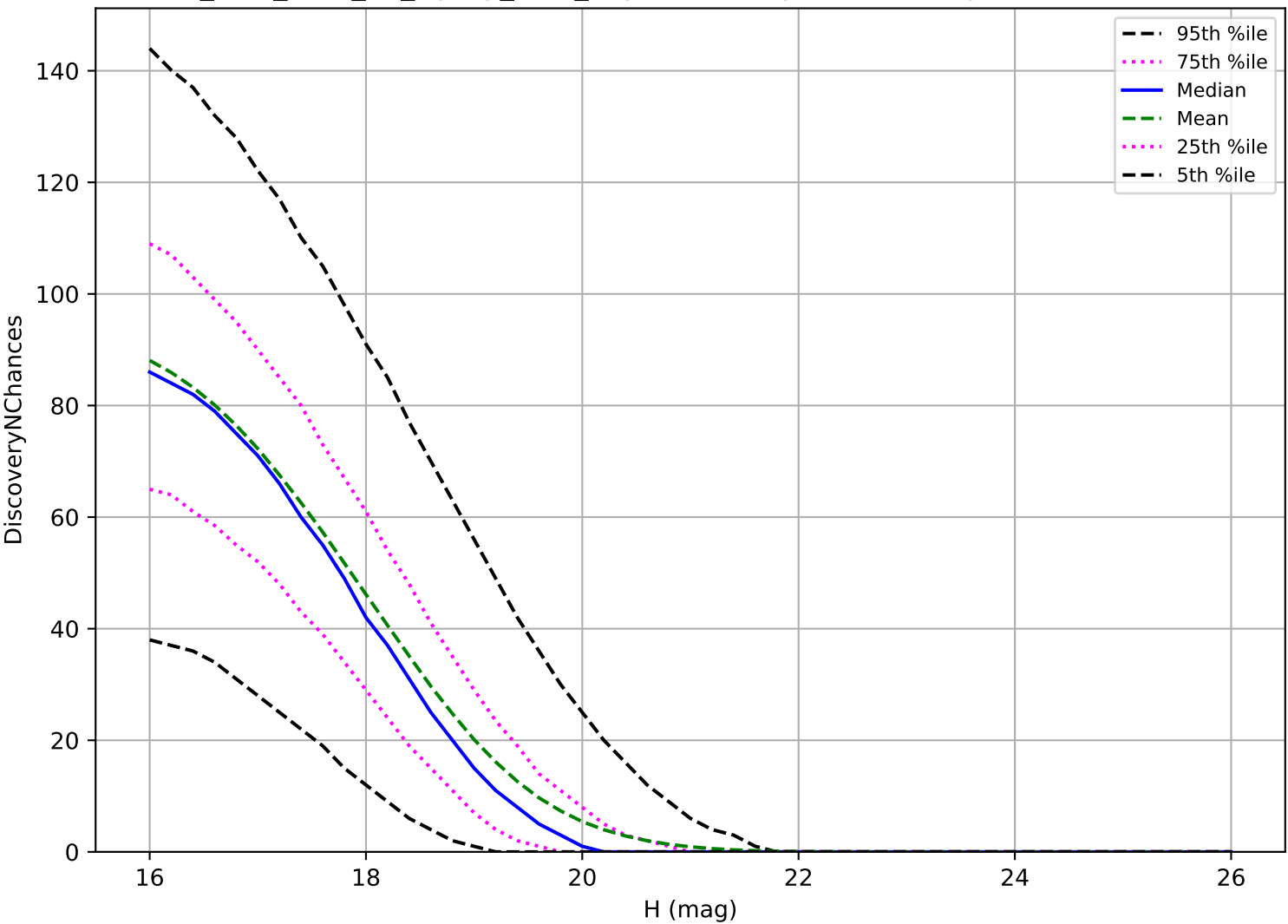
too_elab_r128_d2_ugrizy_v3.4_10yrs: MBA 3 pairs in 15 nights detection loss
