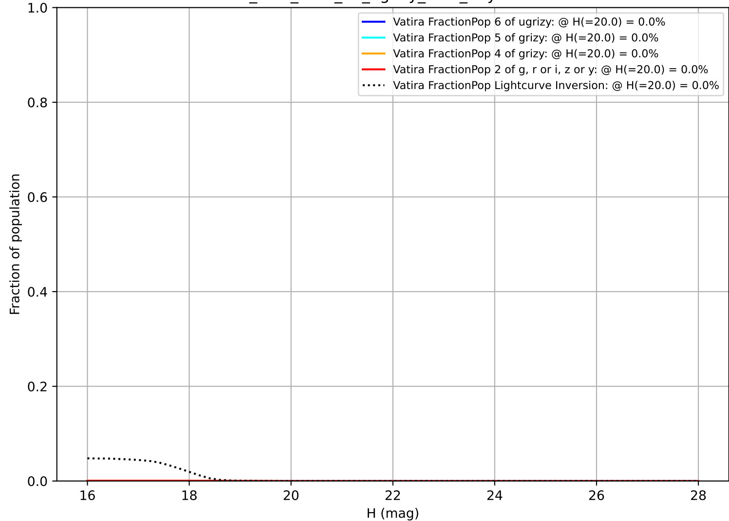
too_elab_r128_d2_ugrizy_v3.4_10yrs Vatira
