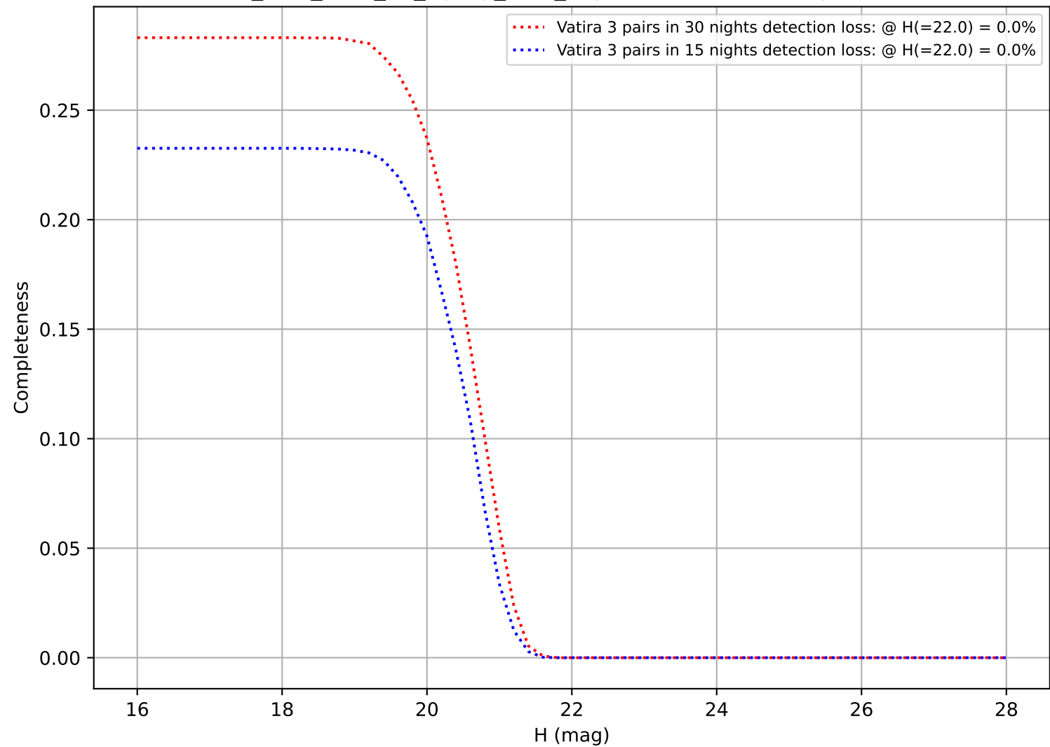
too_elab_r128_d2_ugrizy_v3.4_10yrs: DifferentialCompleteness
