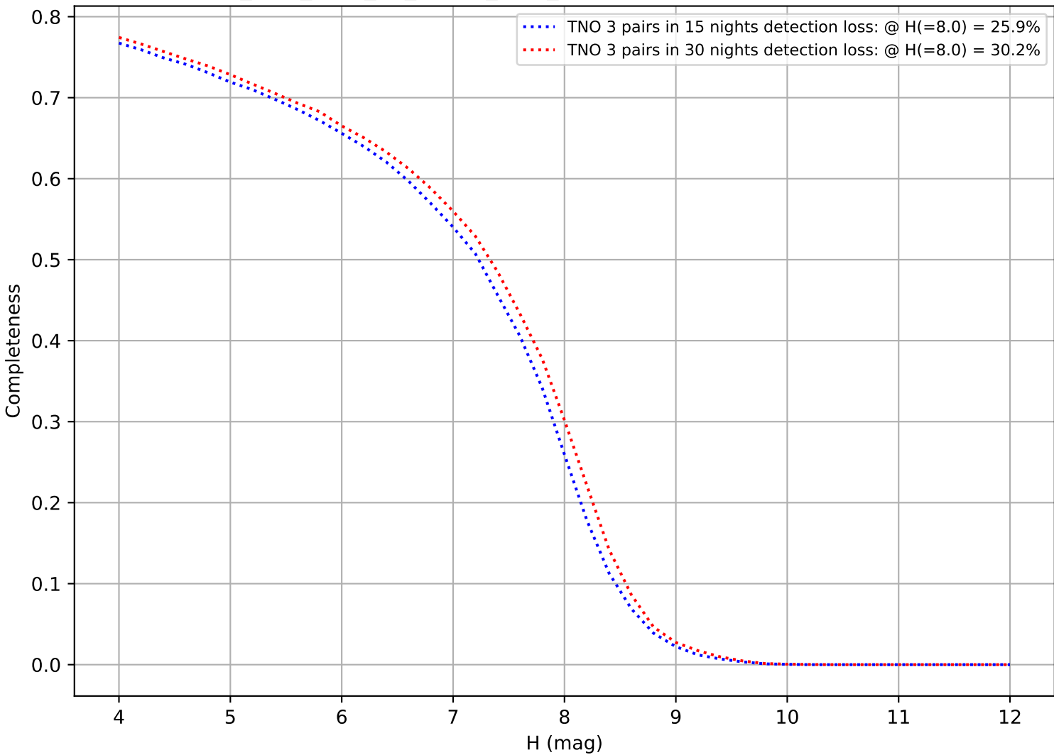
too_elab_r128_d2_ugrizy_v3.4_10yrs: DifferentialCompleteness
