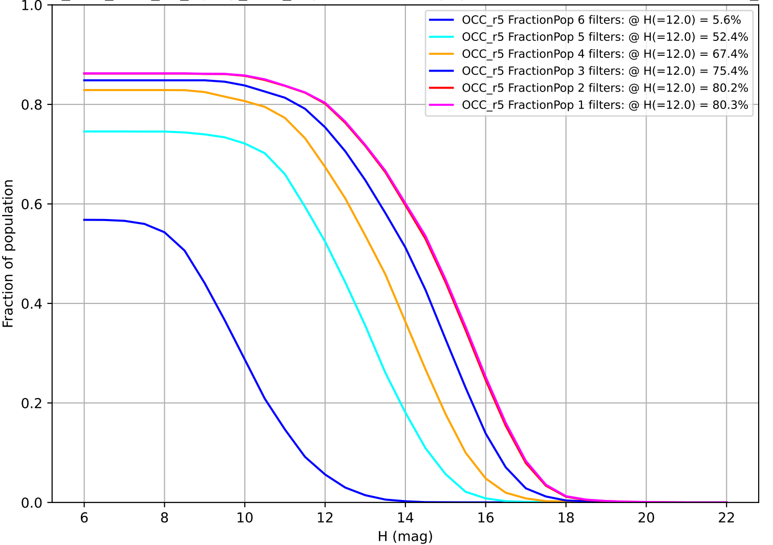
too_elab_r128_d2_ugrizy_v3.4_10yrs: Fraction of population with colors in X filters OCC_r5
