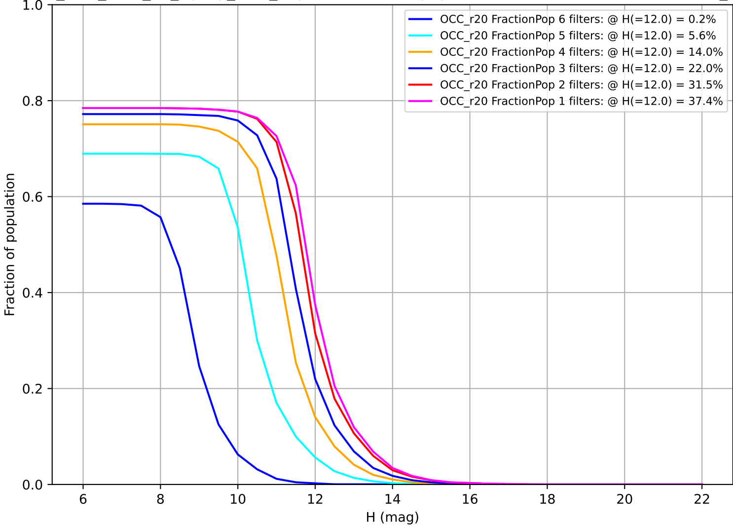
too_elab_r128_d2_ugrizy_v3.4_10yrs: Fraction of population with colors in X filters OCC_r20
