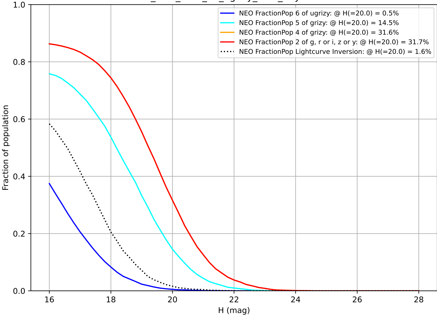
too_elab_r128_d2_ugrizy_v3.4_10yrs NEO
