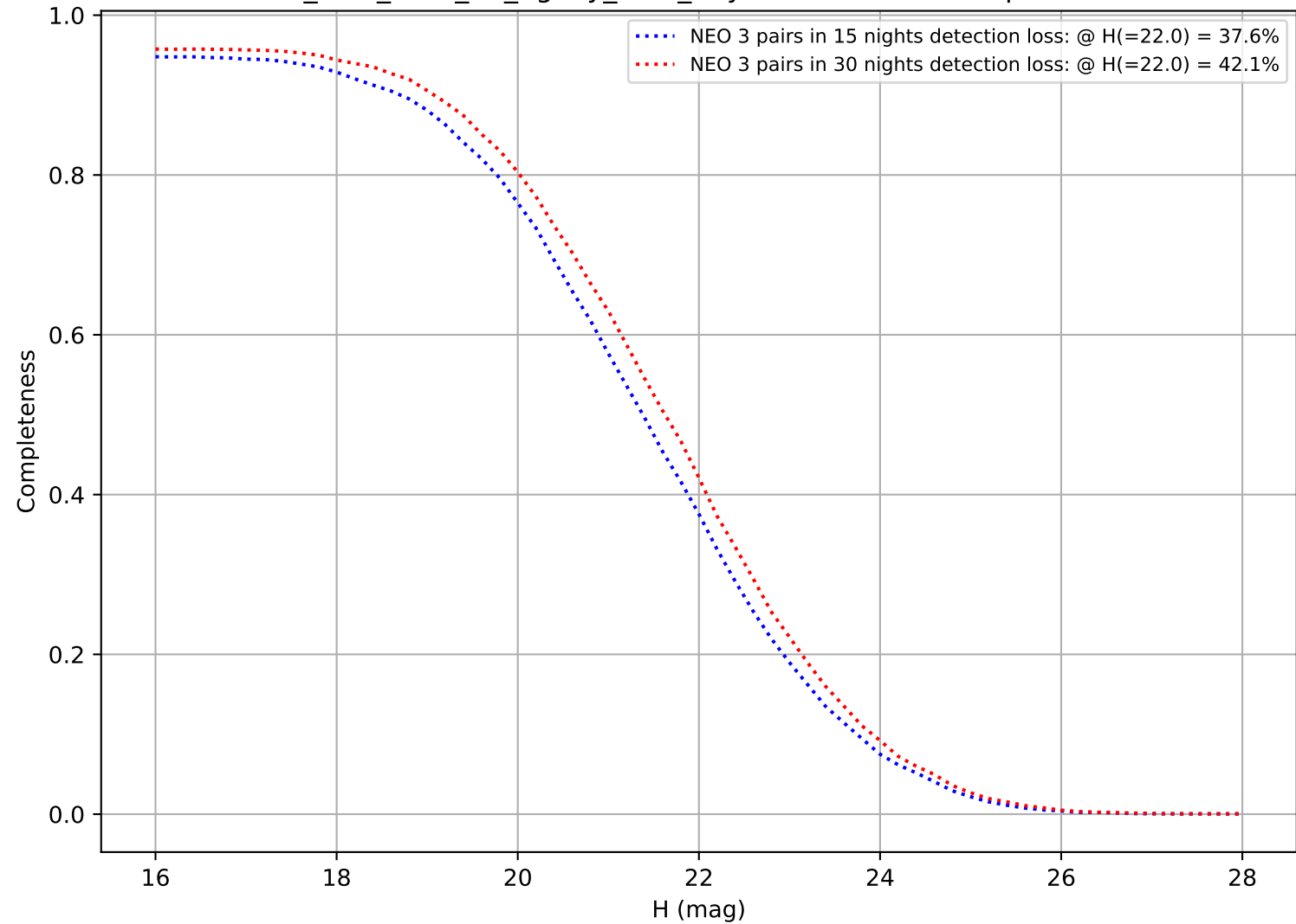
too_elab_r128_d2_ugrizy_v3.4_10yrs: DifferentialCompleteness
