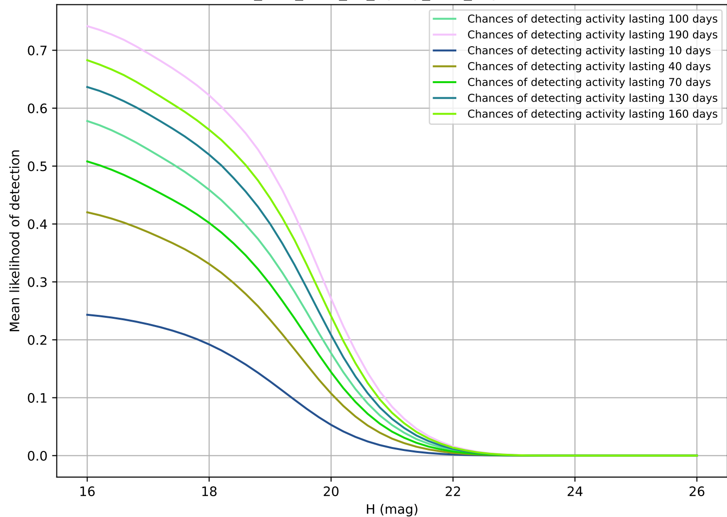
too_elab_r128_d2_ugrizy_v3.4_10yrs MBA
