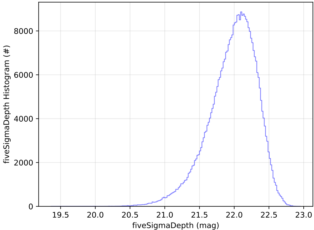
too_elab_r128_d2_ugrizy_v3.4_10yrs y: fiveSigmaDepth Histogram
