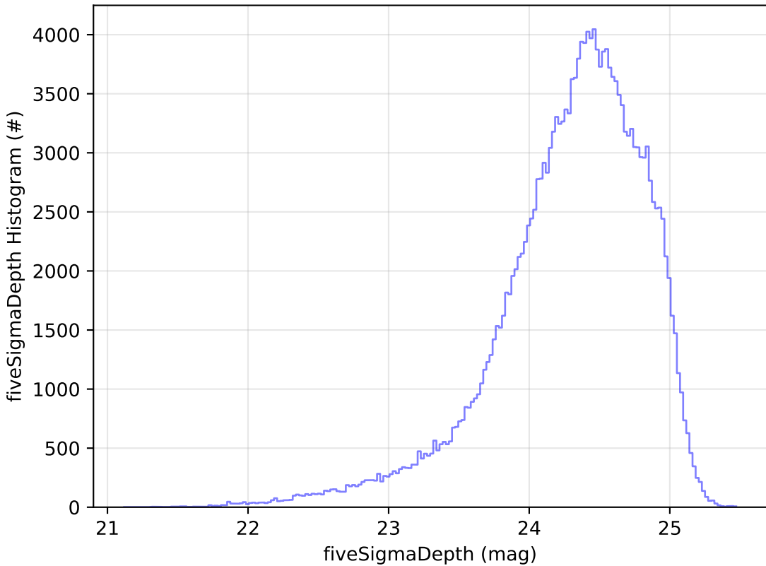
too_elab_r128_d2_ugrizy_v3.4_10yrs g: fiveSigmaDepth Histogram
