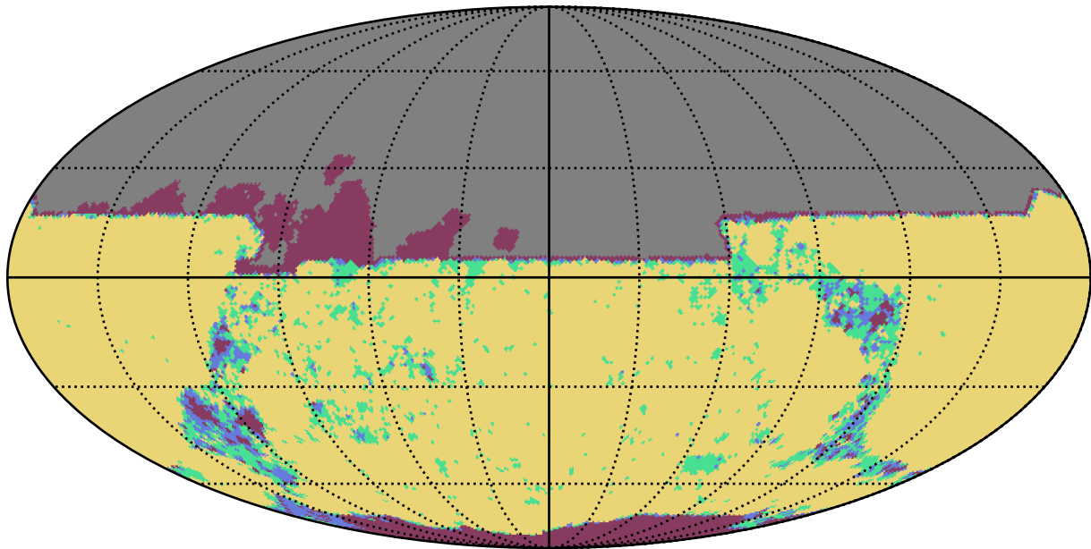
too_elab_r128_d2_ugrizy_v3.4_10yrs y band: YearCoverage night
