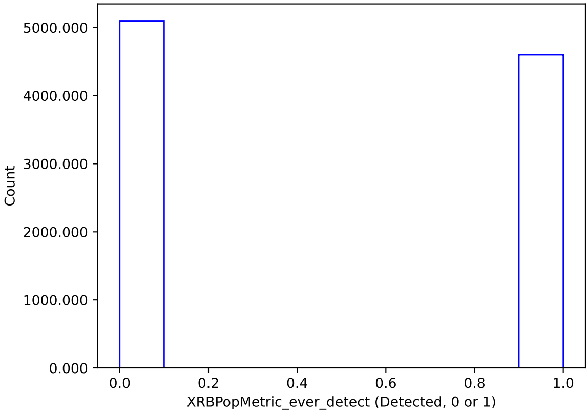
too_elab_r128_d2_ugrizy_v3.4_10yrs : XRBPoMetric_ever_detect
