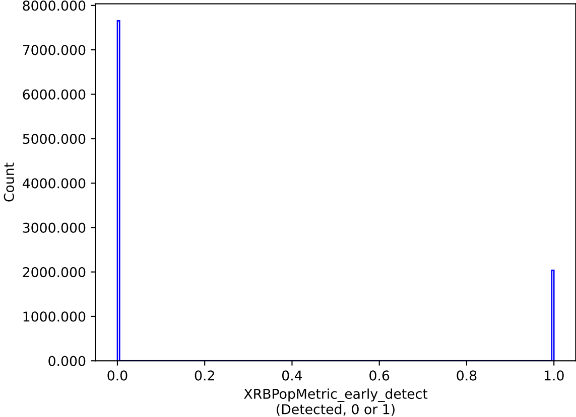
too_elab_r128_d2_ugrizy_v3.4_10yrs : XRBPopMetric_early_detect
