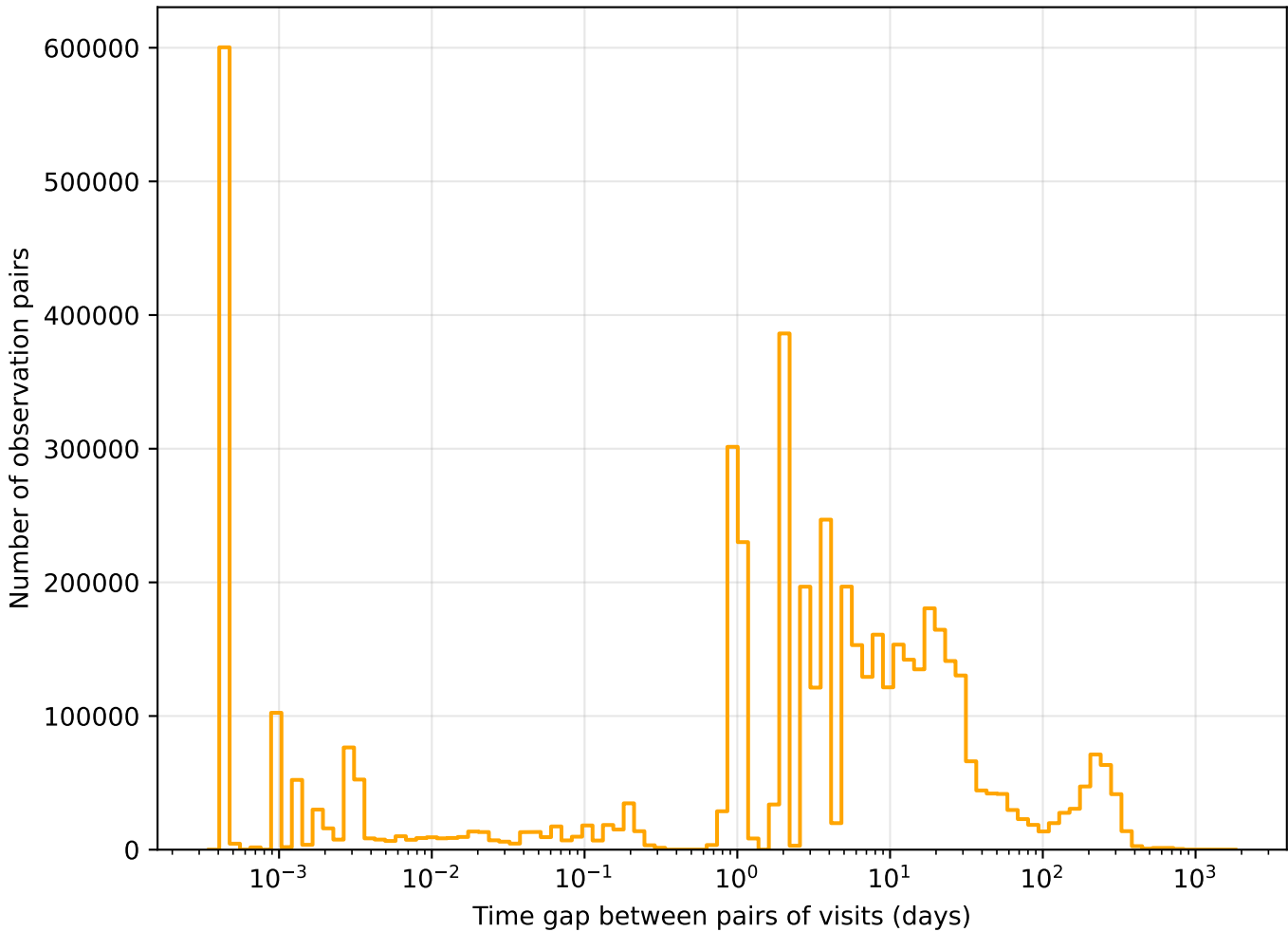
too_elab_r128_d2_ugrizy_v3.4_10yrs r band: Tgaps observationStartMJD
