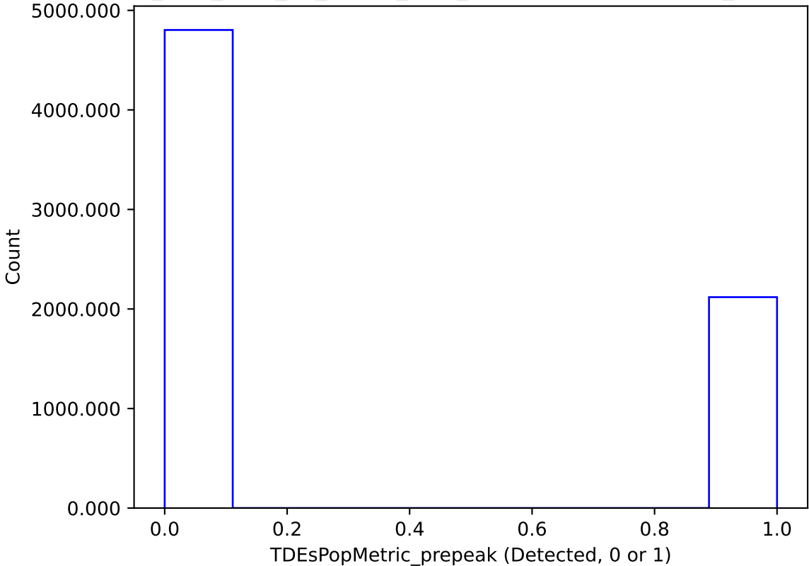
too_elab_r128_d2_ugrizy_v3.4_10yrs : TDEsPopMetric_prepeak
