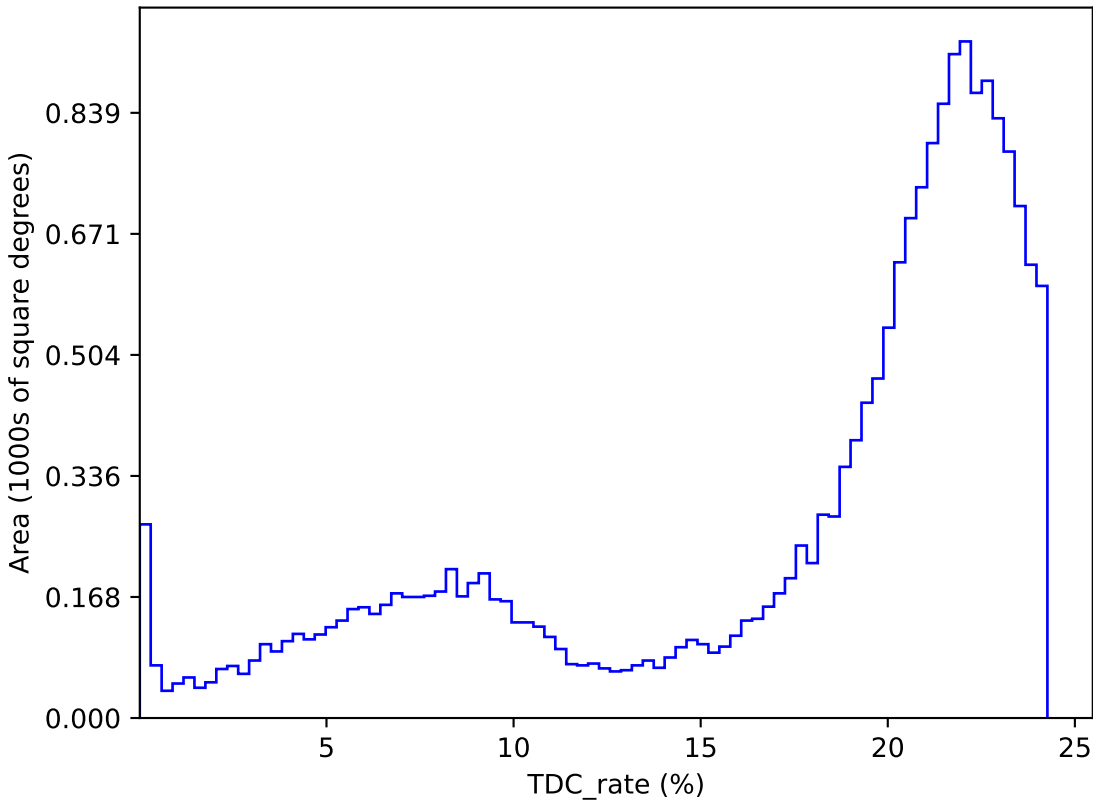
too_elab_r128_d2_ugrizy_v3.4_10yrs : TDC_rate
