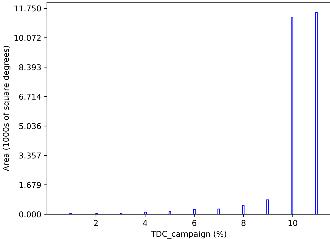
too_elab_r128_d2_ugrizy_v3.4_10yrs : TDC_campaign
