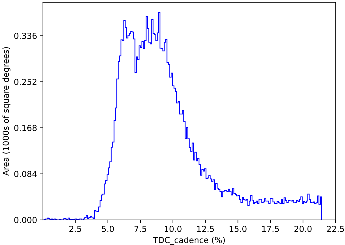
too_elab_r128_d2_ugrizy_v3.4_10yrs : TDC_cadence
