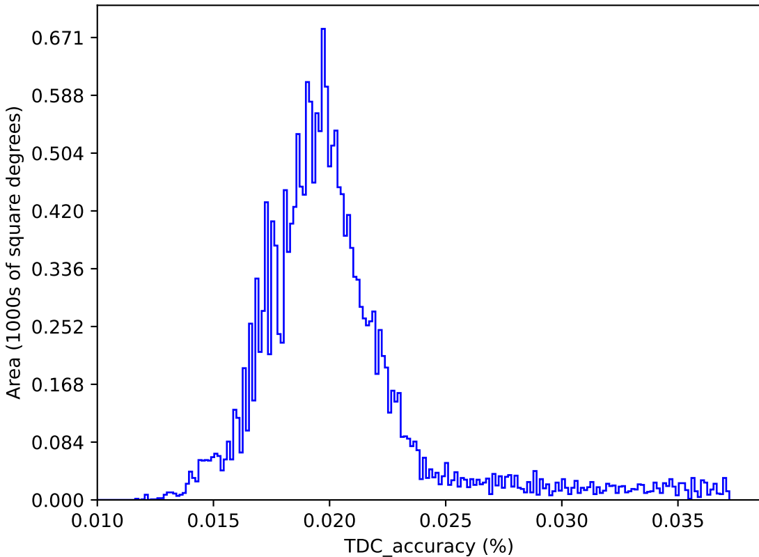
too_elab_r128_d2_ugrizy_v3.4_10yrs : TDC_accuracy
