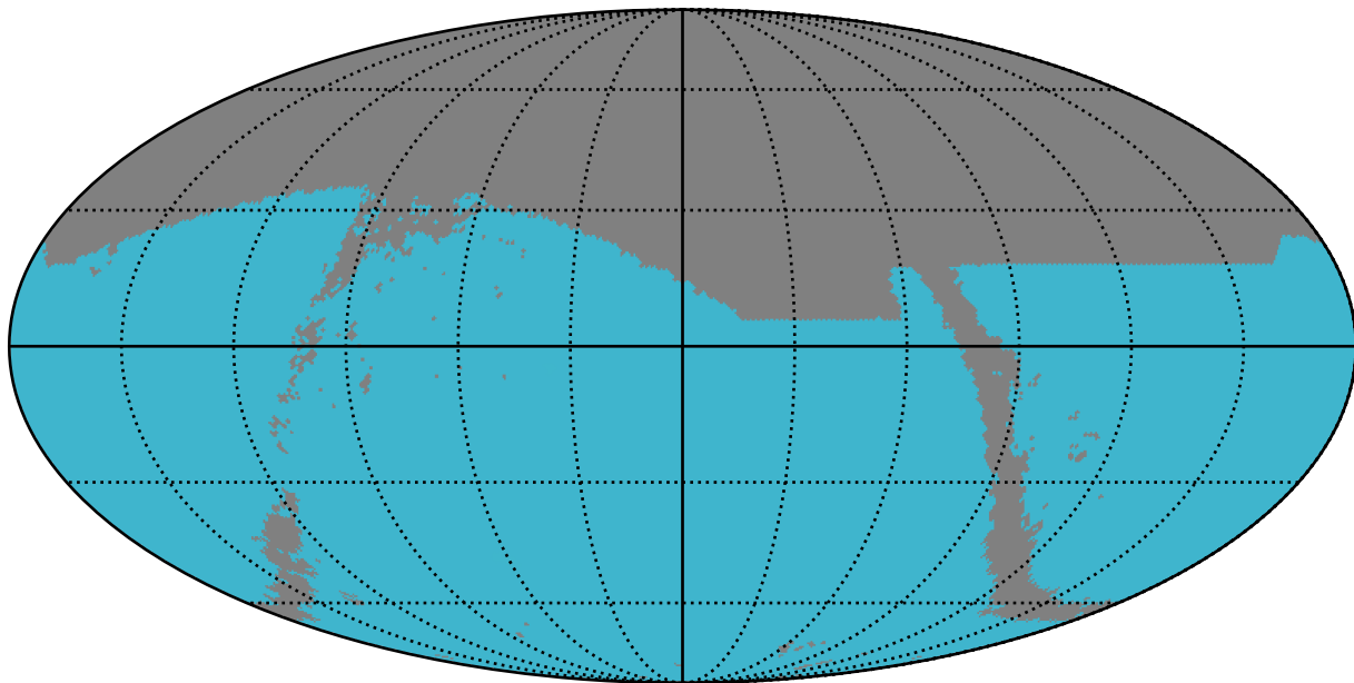
too_elab_r128_d2_ugrizy_v3.4_10yrs : SNSLMetric
