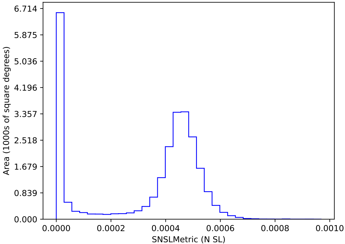
too_elab_r128_d2_ugrizy_v3.4_10yrs : SNSLMetric
