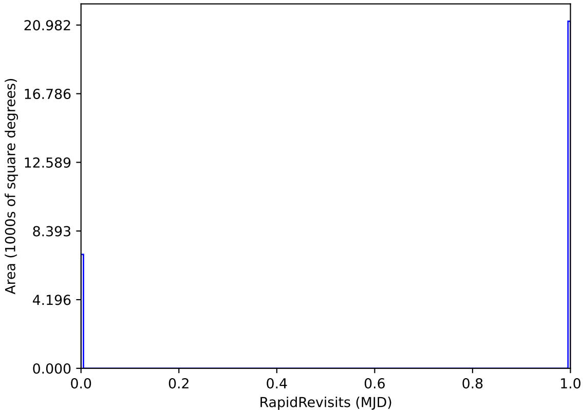
too_elab_r128_d2_ugrizy_v3.4_10yrs : RapidRevisits
