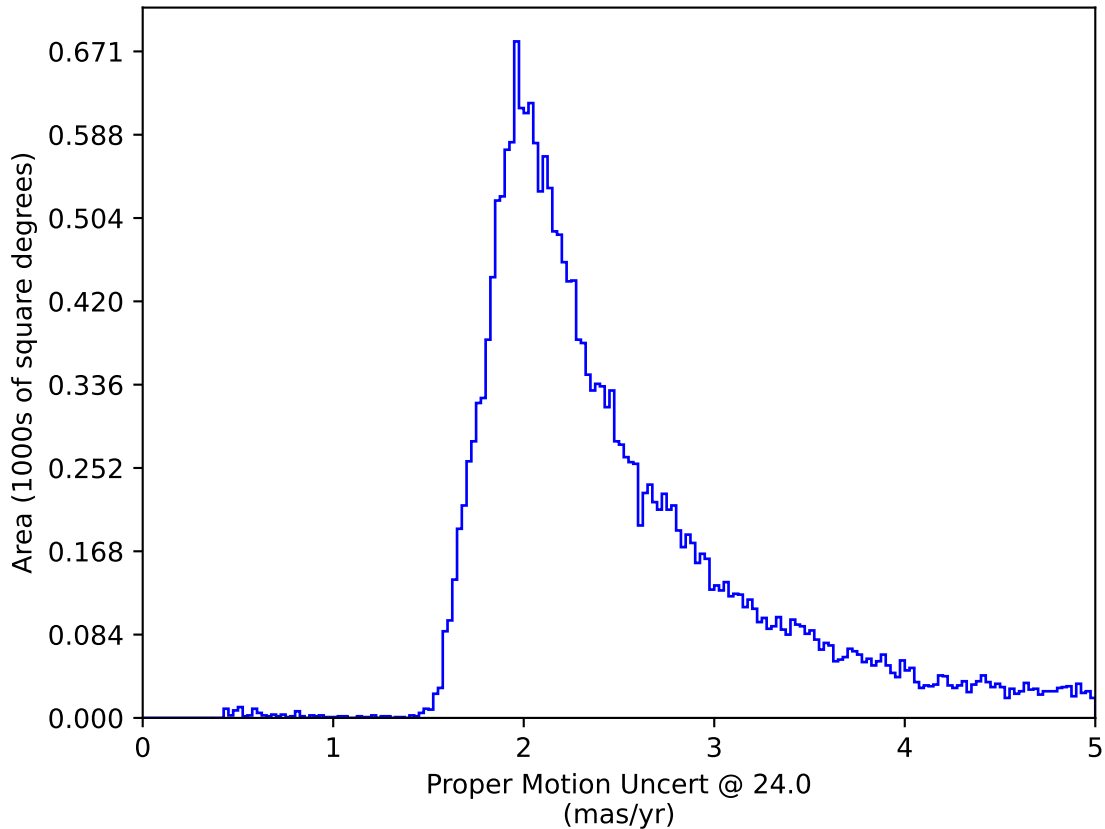
too_elab_r128_d2_ugrizy_v3.4_10yrs : Proper Motion Uncert @ 24.0
