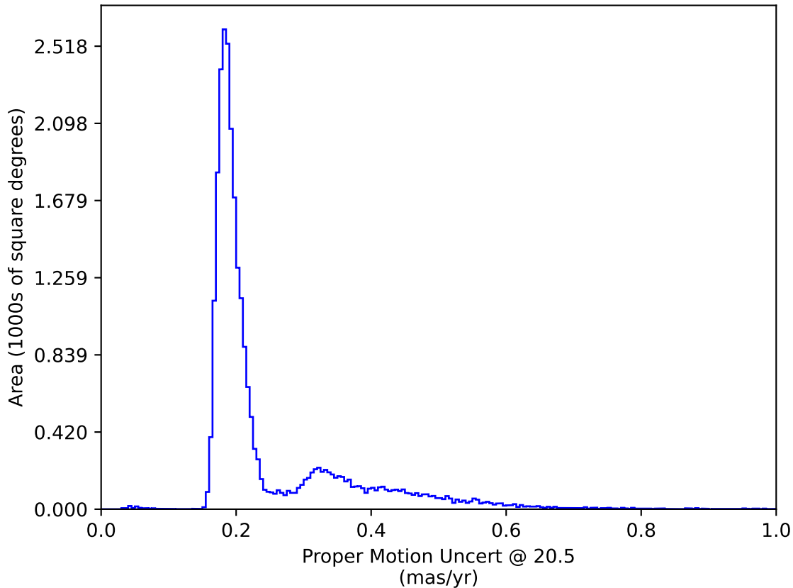
too_elab_r128_d2_ugrizy_v3.4_10yrs : Proper Motion Uncert @ 20.5
