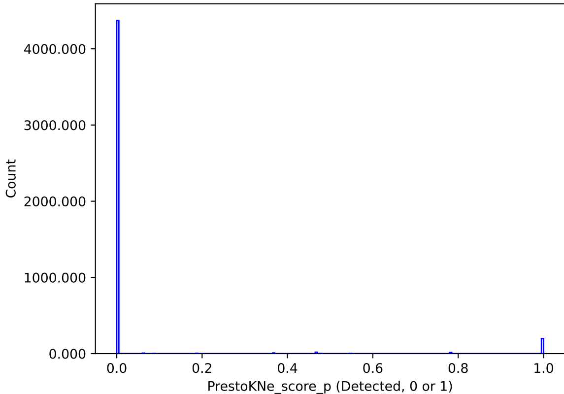
too_elab_r128_d2_ugrizy_v3.4_10yrs : PrestoKNe_score_p
