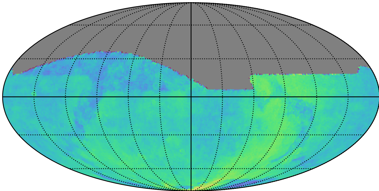
too_elab_r128_d2_ugrizy_v3.4_10yrs : Parallax Coverage @ 24.0
