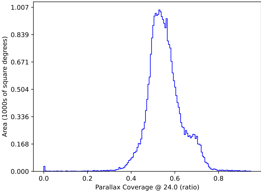
too_elab_r128_d2_ugrizy_v3.4_10yrs : Parallax Coverage @ 24.0
