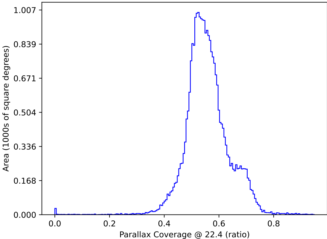
too_elab_r128_d2_ugrizy_v3.4_10yrs : Parallax Coverage @ 22.4
