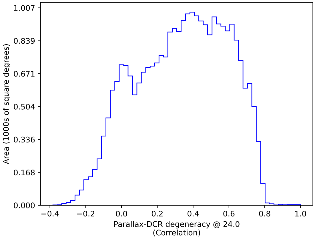
too_elab_r128_d2_ugrizy_v3.4_10yrs : Parallax-DCR degeneracy @ 24.0
