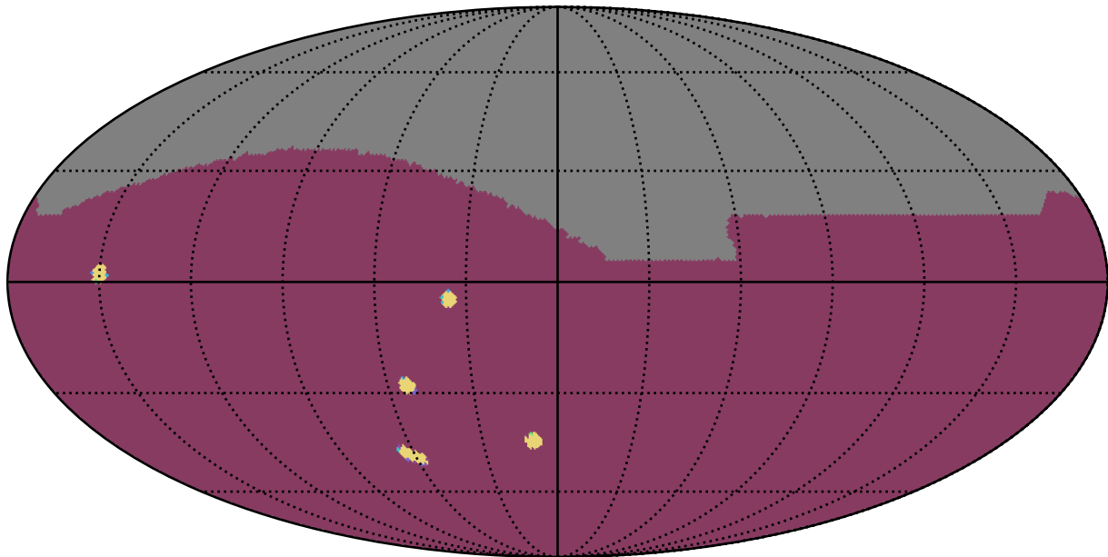
too_elab_r128_d2_ugrizy_v3.4_10yrs : NumberOfQuickRevisits
