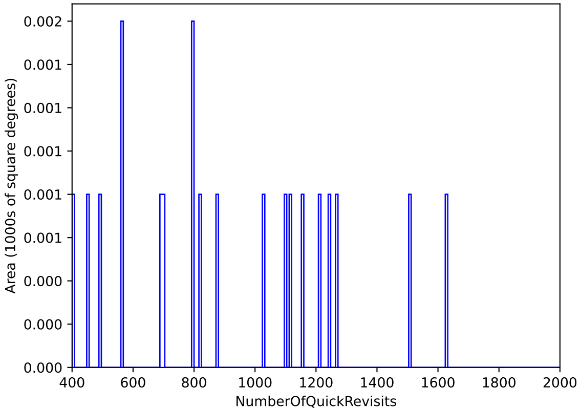
too_elab_r128_d2_ugrizy_v3.4_10yrs : NumberOfQuickRevisits
