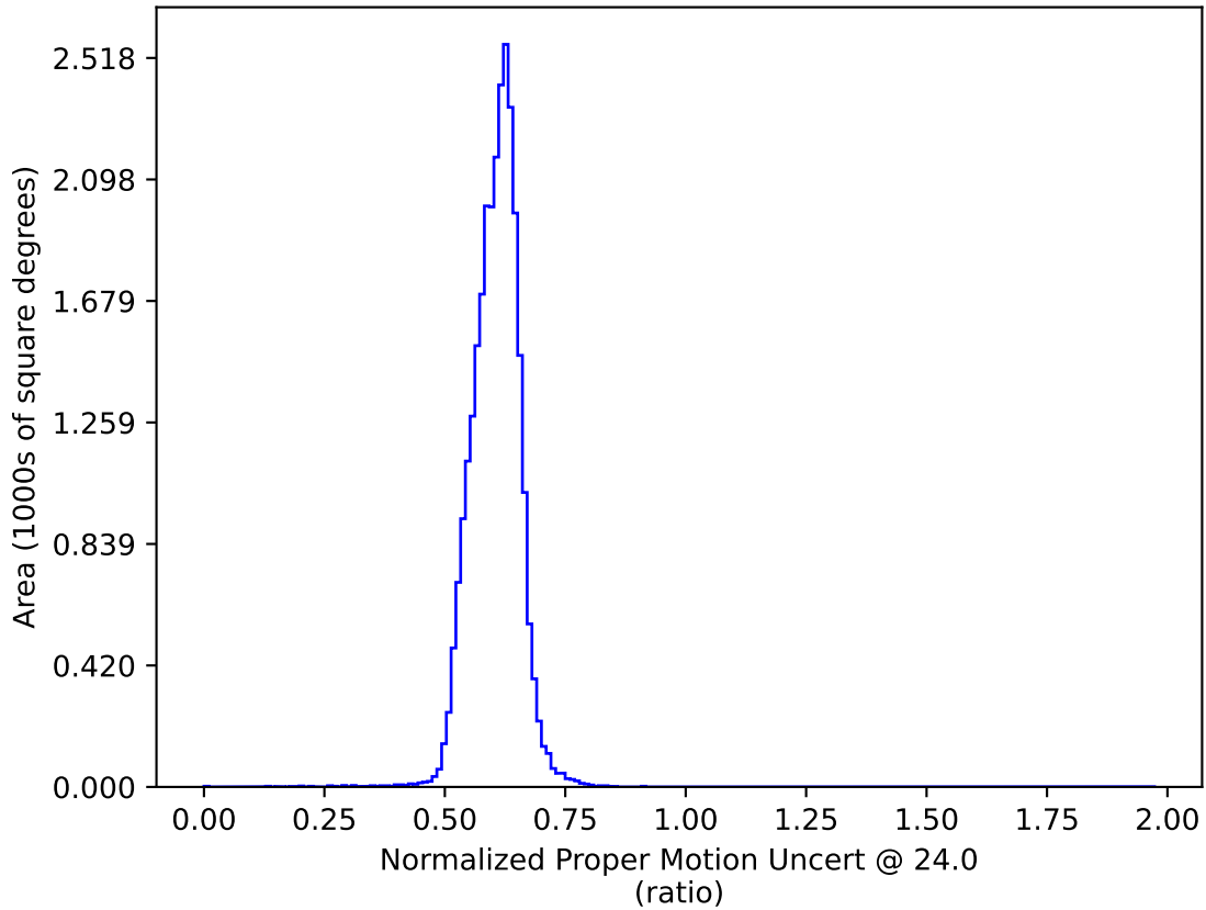
too_elab_r128_d2_ugrizy_v3.4_10yrs : Normalized Proper Motion Uncert @ 24.0
