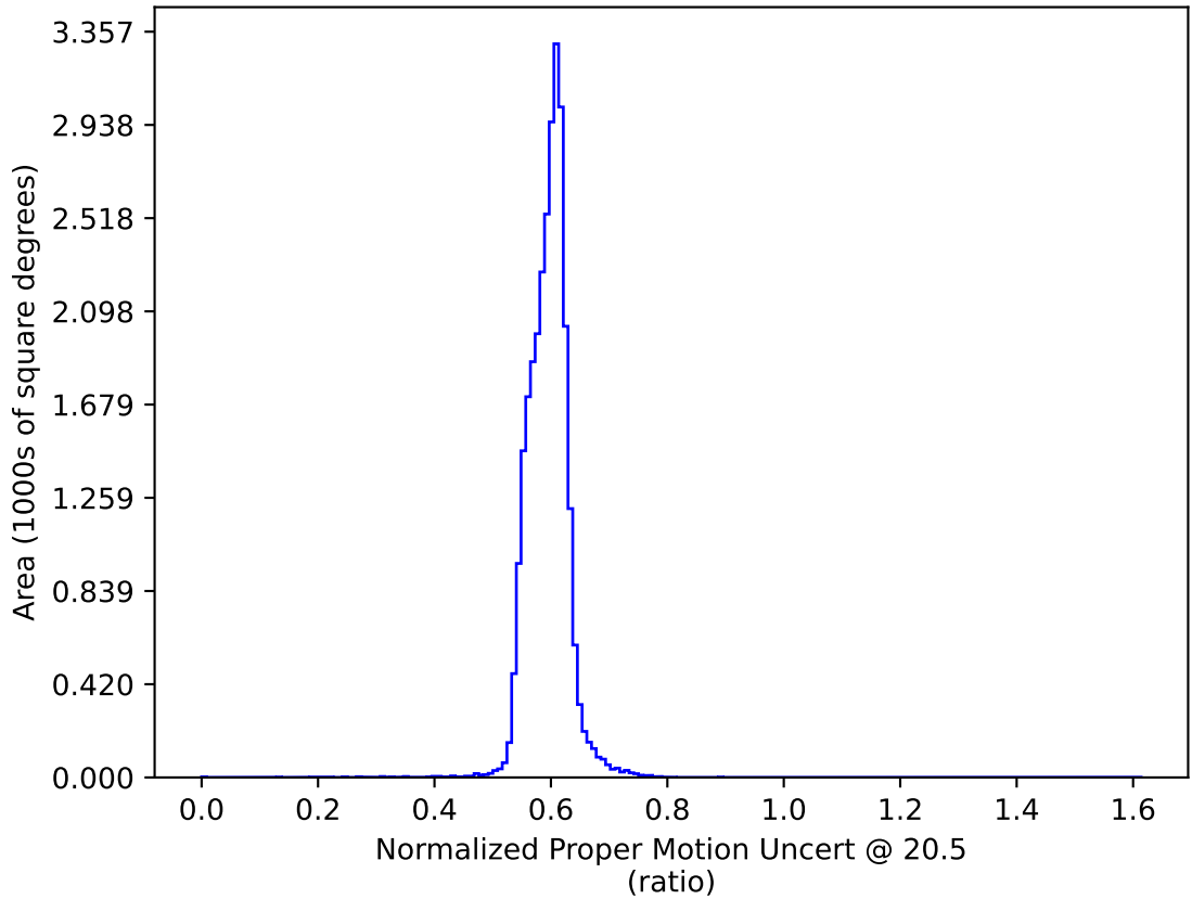
too_elab_r128_d2_ugrizy_v3.4_10yrs : Normalized Proper Motion Uncert @ 20.5
