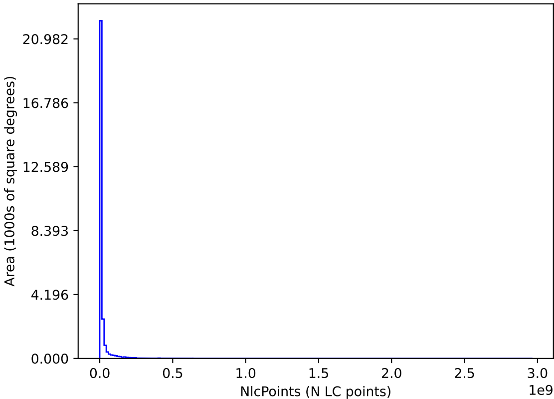
too_elab_r128_d2_ugrizy_v3.4_10yrs : NlcPoints
