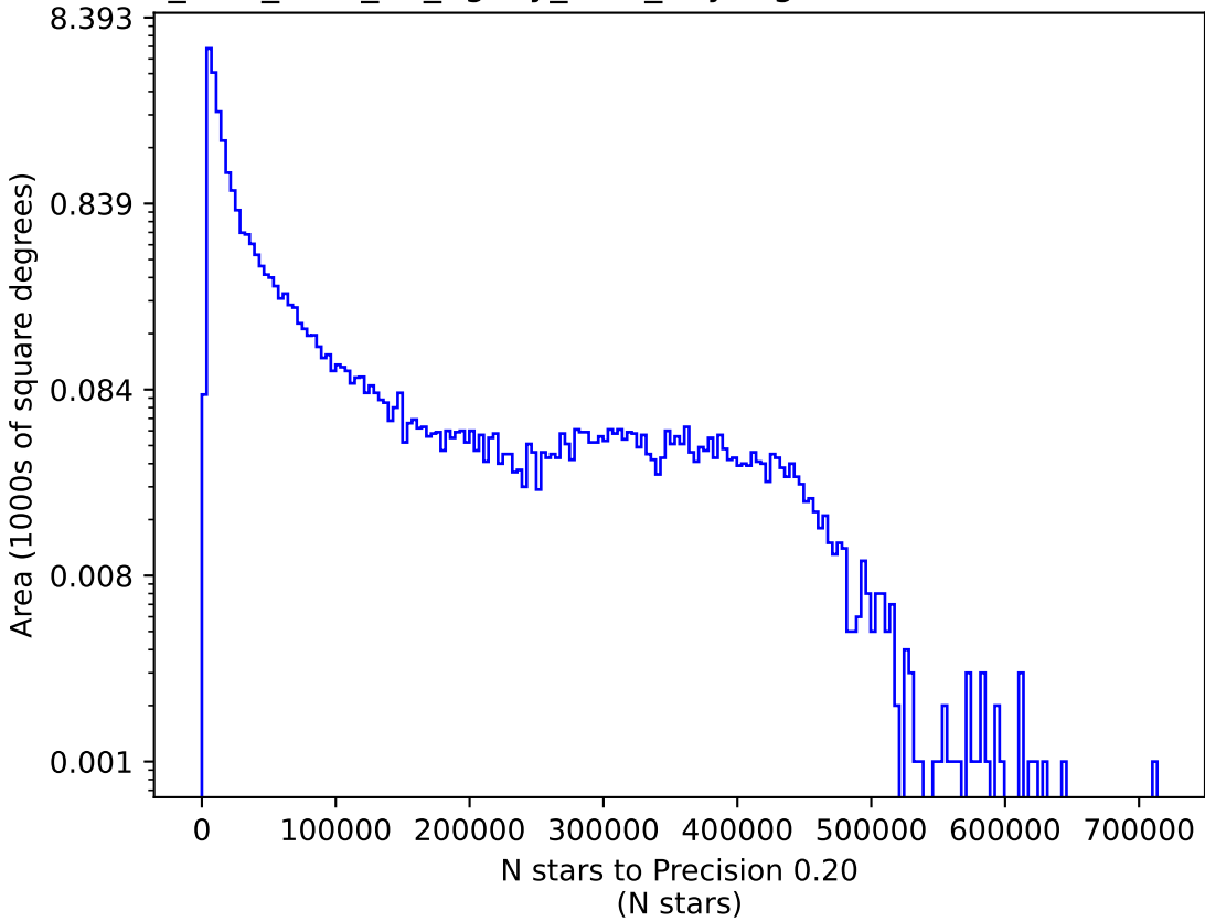
too_elab_r128_d2_ugrizy_v3.4_10yrs g: N stars to Precision 0.20
